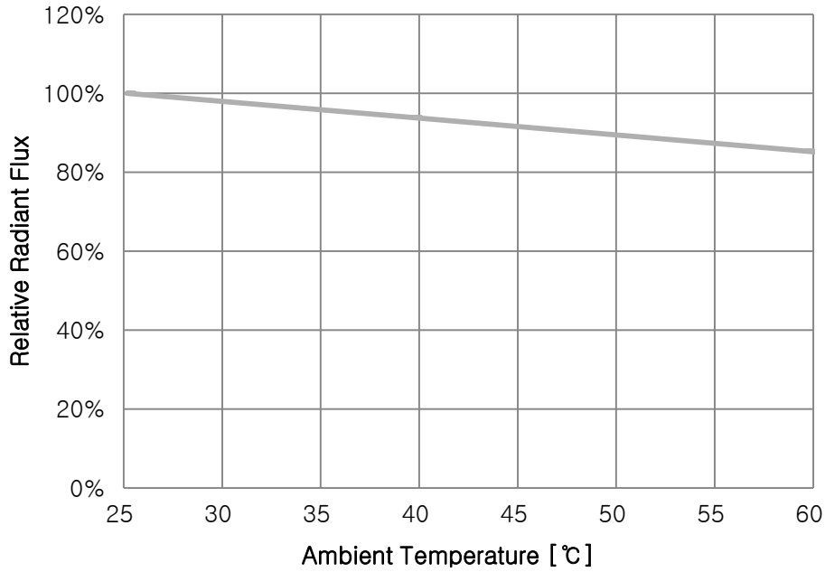
Fig 5. Ambient Temperature vs. Relative Radiant Flux, I_F=20\text{mA}
