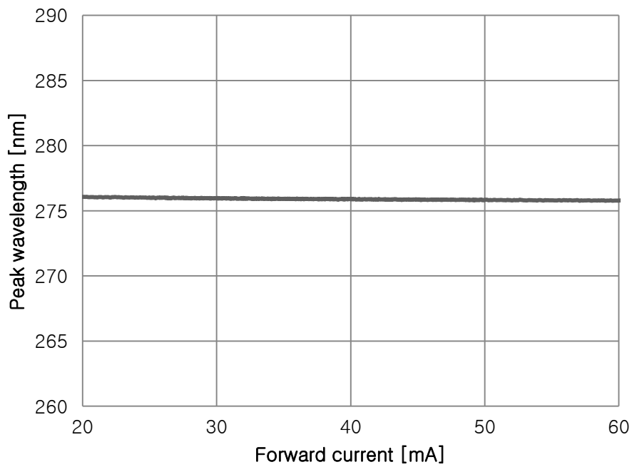
Fig 4. Forward Current vs. Peak Wavelength, T_a=25^\circ\text{C}
