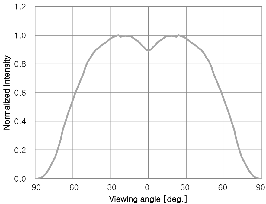
Fig 8. Typical Spatial Distribution, I_F=20\text{mA}
