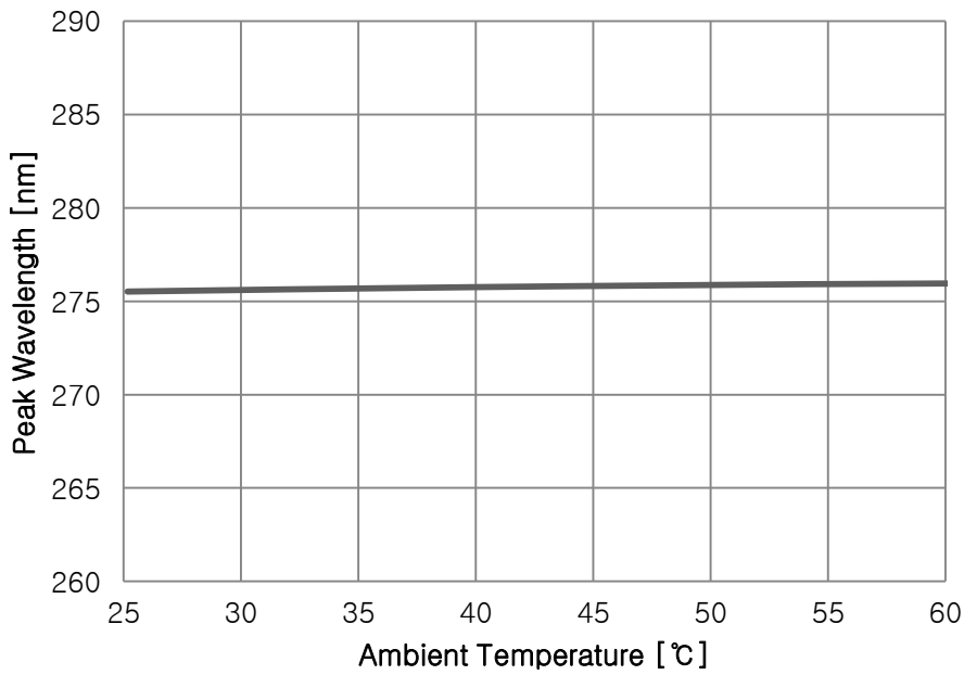
Fig 6. Ambient Temperature vs. Peak Wavelength, I_F=20\text{mA}
